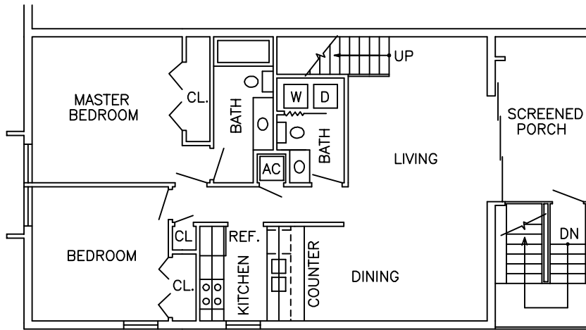
1st FLOOR PLAN—BLDGS.1,2,3,4,7 & 8
